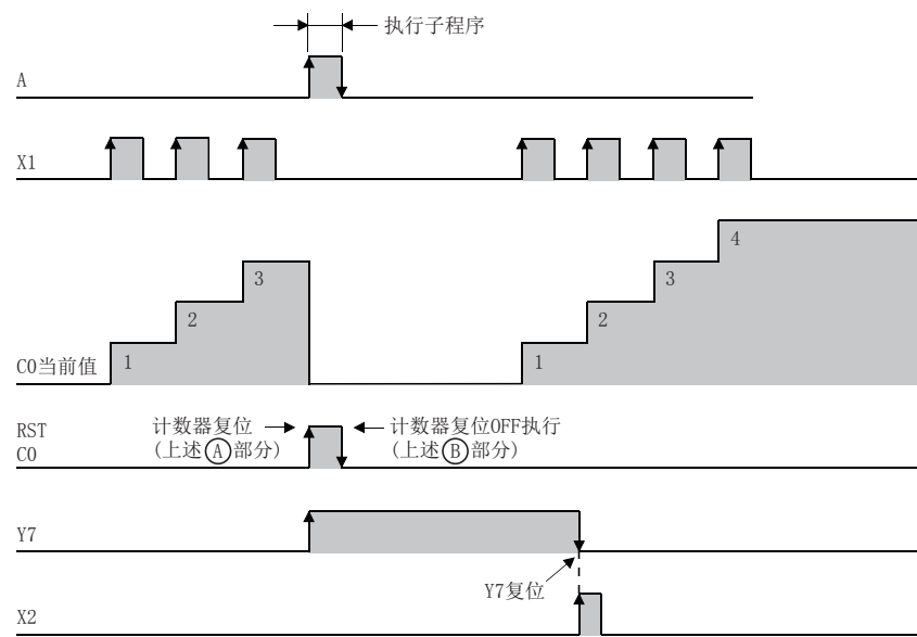
[时序图]
