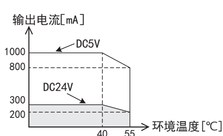
■FX3U-1PSU-5V
