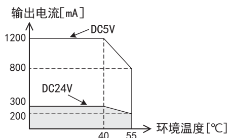
■FX5-1PSU-5V
