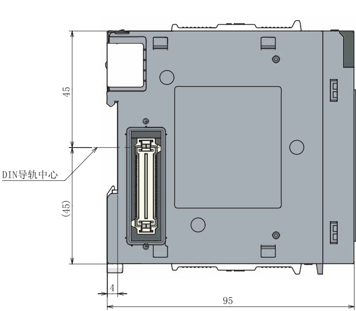
[6] LD75D4
