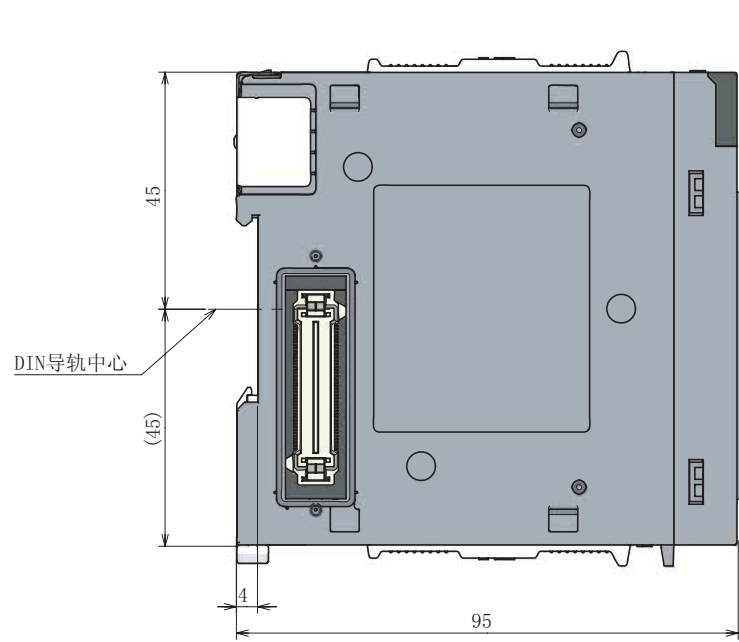
[3] LD75P4
